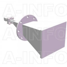
LB-28-25-C2-EKFSP0 Standard Gain Horn Antenna 26.5-40GHz 25dB Gain 2.92mm Female
